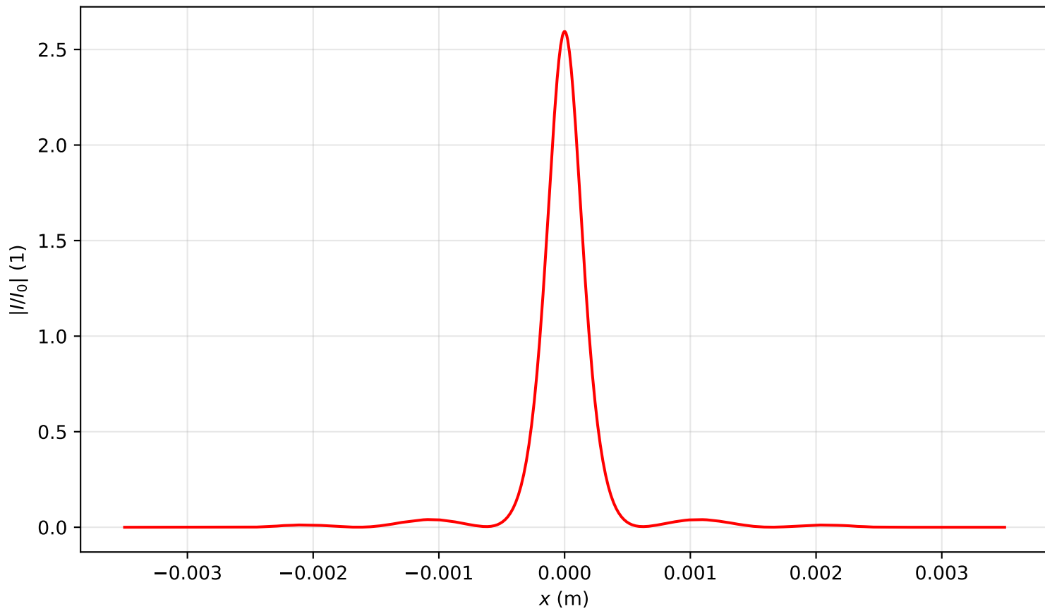
Intensity profile I(x, y = 0, z = 0.796)/I_0 , P_{in}=1.0P_{cr} , artificial time
